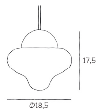
NUTTY GOLD OR BLACK BASE CLEAR OR COLORED GLASS H175 X W186 CM
