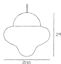
NUTTY XL GOLD OR BLACK BASE CLEAR OR COLORED GLASS H290 X W301 CM
